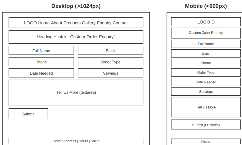
Figure 4: Custom Order Enquiry page wireframe (desktop and mobile)
