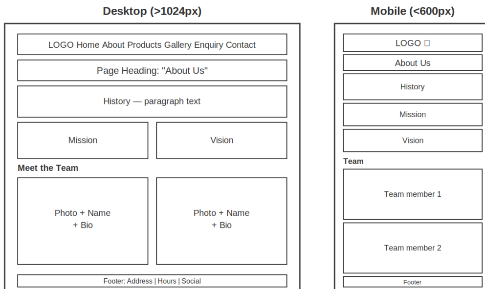
Figure 2: About Us page wireframe (desktop and mobile)
