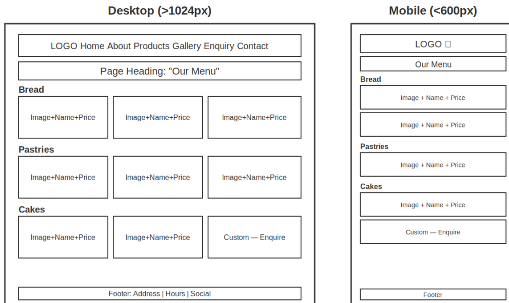
Figure 3: Products/Menu page wireframe (desktop and mobile)
